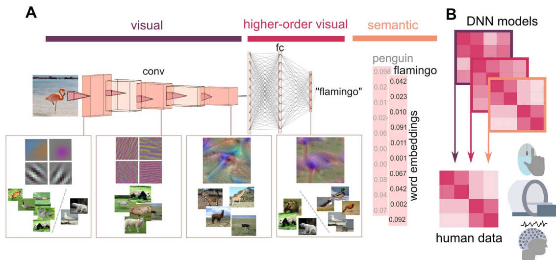
Fig. 1 Linking representational formats in DNNs and in semantic representations to representations in the human brain. A Different representational formats in convolutional deep neural networks (cDNNs) and deep natural language processing models (dNLPs). In cDNNs, images are processed with a gradient in complexity, comparable to the human ventral visual pathway. As in the brain, basic visual information is processed in the first layer (whose receptive field properties roughly match those of V1) and is then passed through the convolutional layers of the network, which process increasingly complex information. After the last convolutional layer, the connections change, as now each neuron is connected to each neuron in subsequent layers (fully-connected). The network then chooses the most active (i.e., most likely) label in the highest layer. Early layers of the cDNN process edges, colors, and textures, such that e.g., animals of different categories (species) are sorted together e.g., based on their color. DNN neu-
